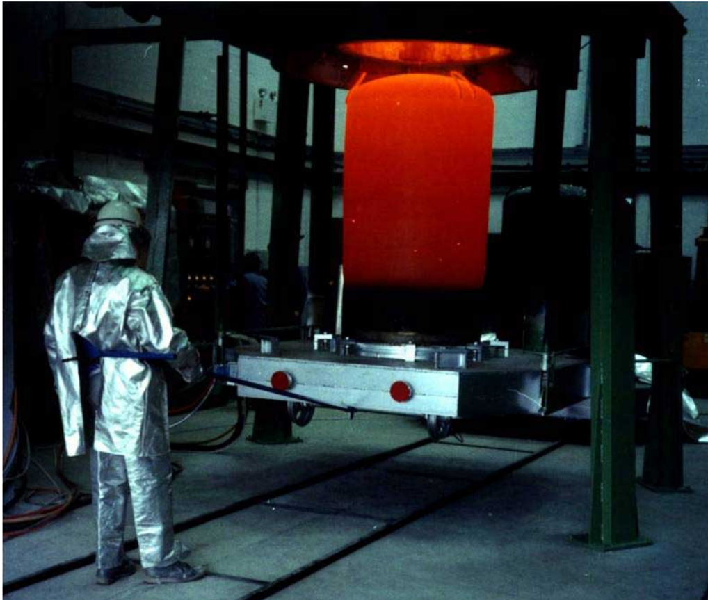
Refurbished Degussa bottom loading Bell furnace with controlled atmosphere cold seal retort. Picture courtesy of ROLLS WOOD GROUP
